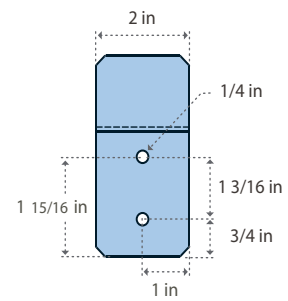
3.0 Z-Bracket (front)
